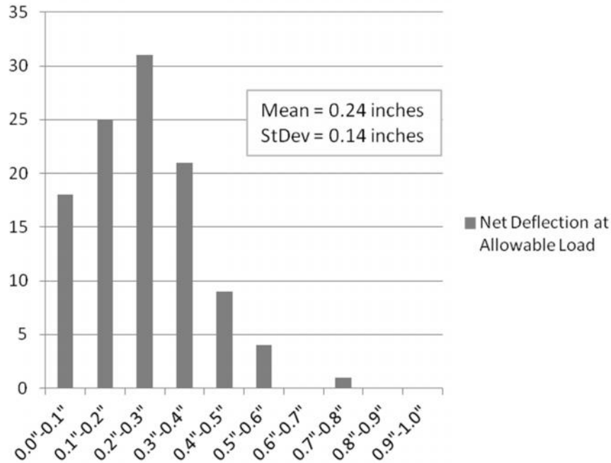
Fig. 9 Net Deflection at Working Capacity for All Tests - Tension Only
